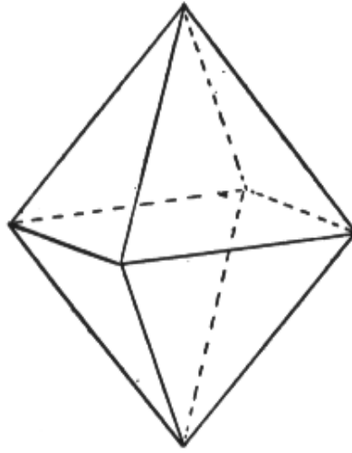
The octahedron
